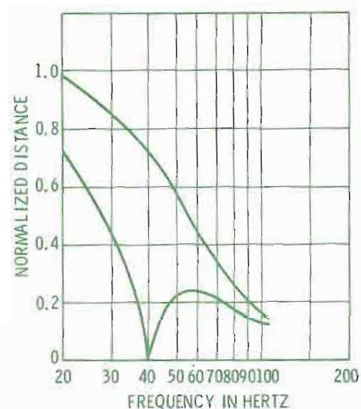
Fig. 7 Cone excursion comparison.
