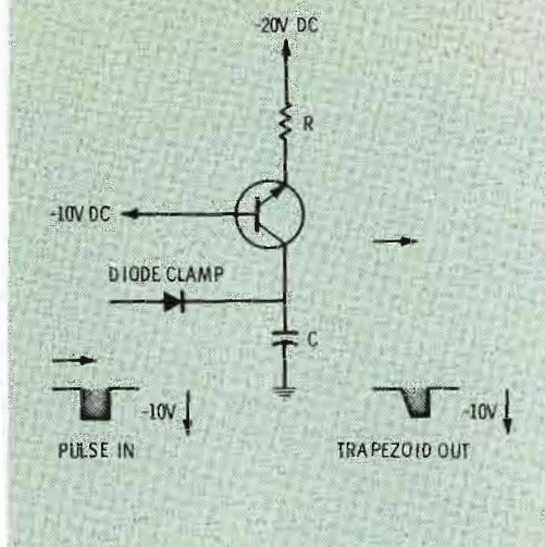
Fig. 5 Typical trapezoid pulse generator in a VTR servo. The diode acts as a clamp to hold the maximum amplitude of the trapezoid to the amplitude of the input pulse.
