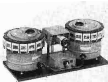
MODEL 332: Newest version of the workhorse of the industry. For monochrome chains; 32-slide capacity. Model 322: single turret for 16 slides, monochrome or color.
